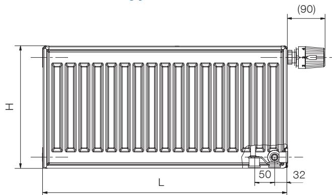
Type 21 VKU
