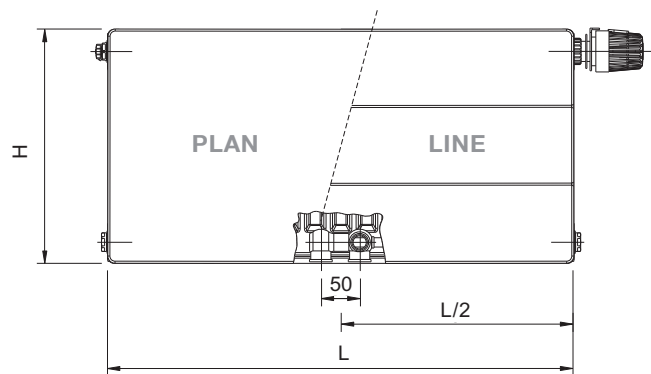
Type 11 PLAN VKM/LINE VKM
